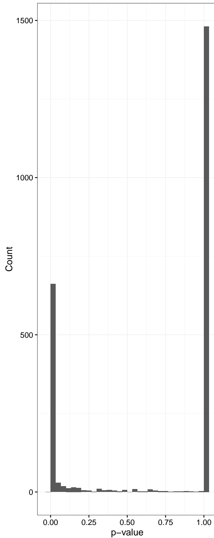
Histogram on adjust p-value without filter
