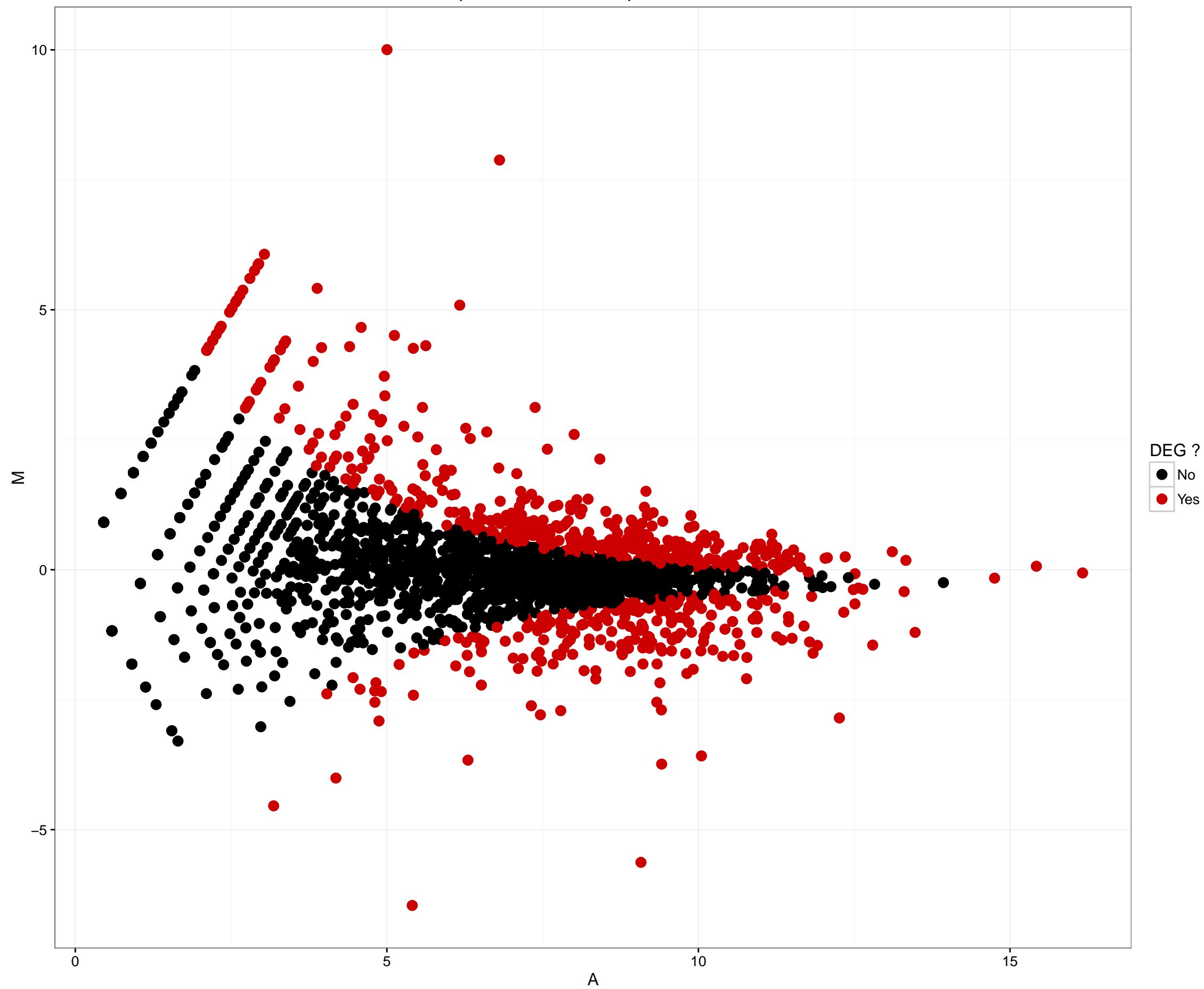
MA plot on normalized pseudo-counts
