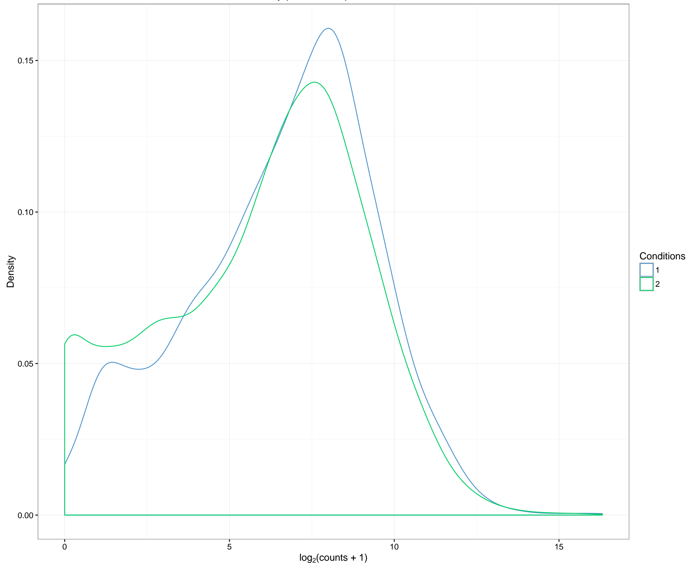
Density plot on raw pseudo-counts
