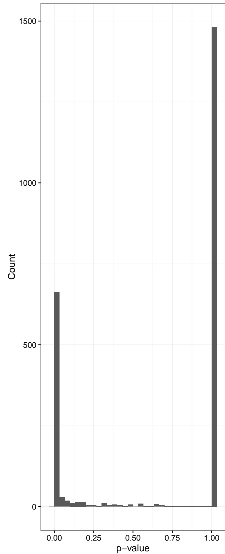
Histogram on adjust p-value with filter
