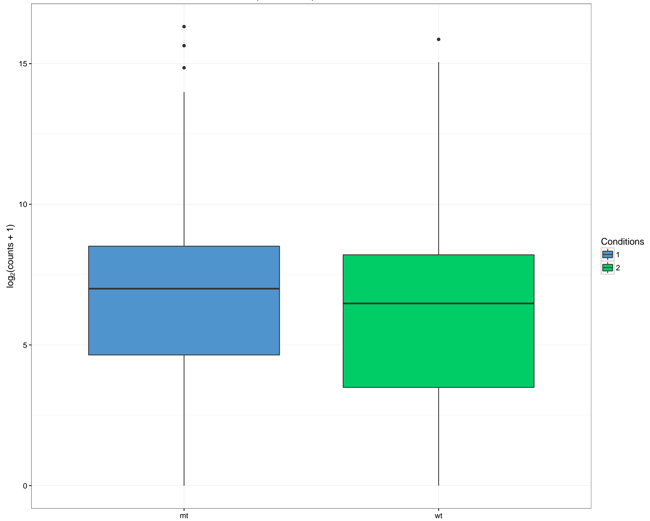
Boxplot on raw pseudo-counts
