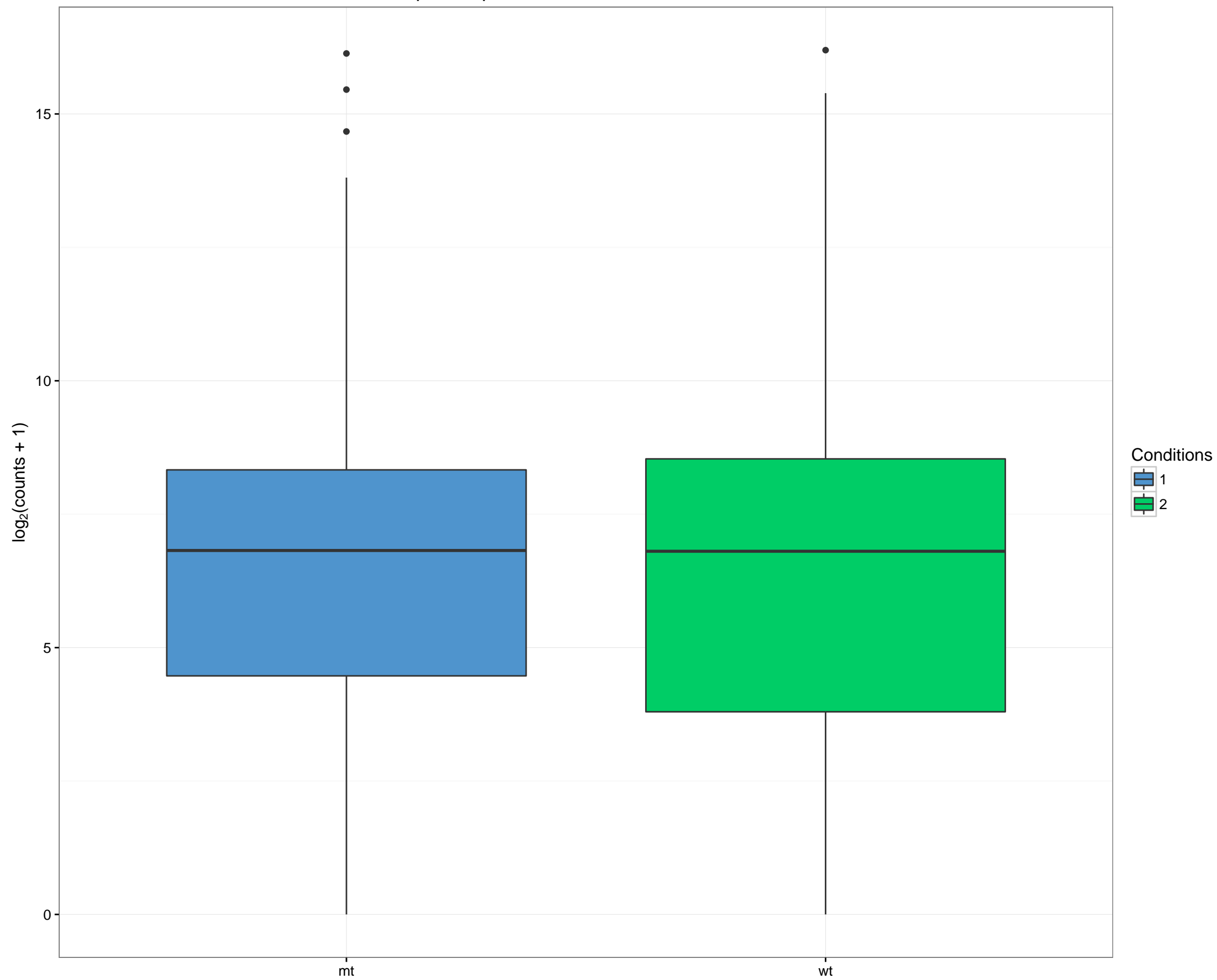
Boxplot on pseudo-counts after normalization
