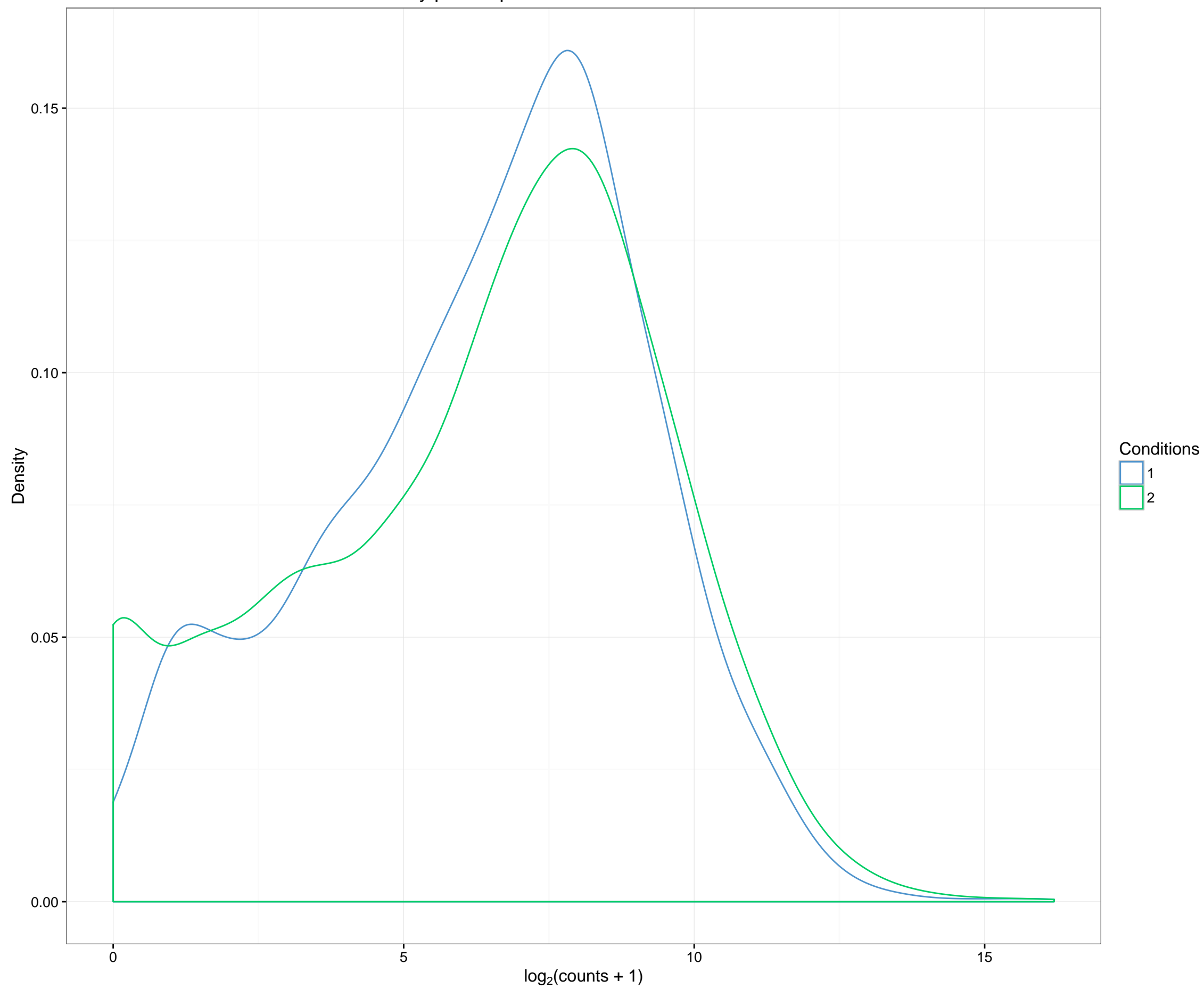
Density plot on pseudo-counts after normalization
