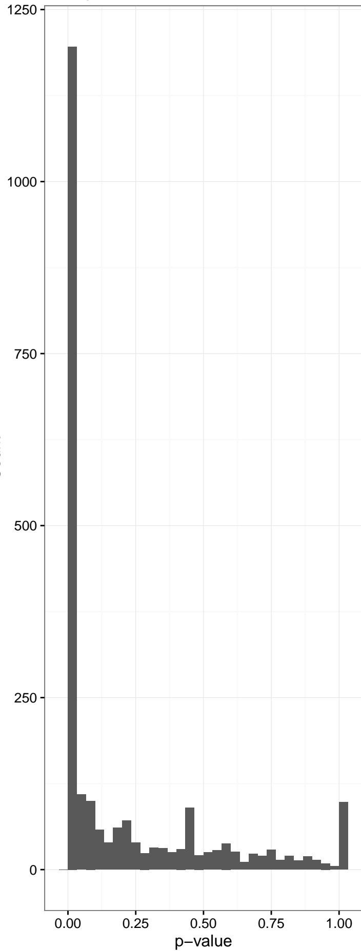
Histogram on raw p-value without filter
